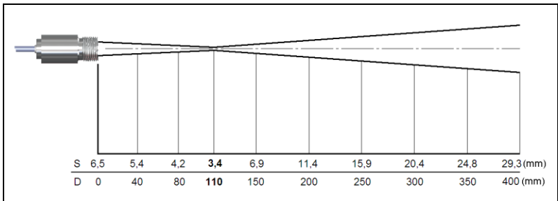
3MH CF D:S = 33:1 / D:S Far field = 11:1
